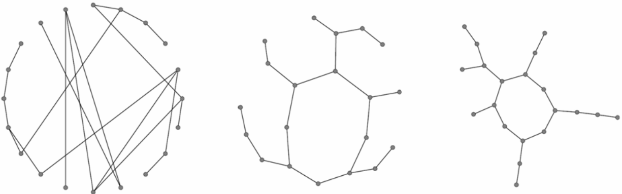
Figure 13. Circle layout (left), Fruchterman-Rheingold layout (middle), and Kamada-Kawai Layout (right) of a small world network.
