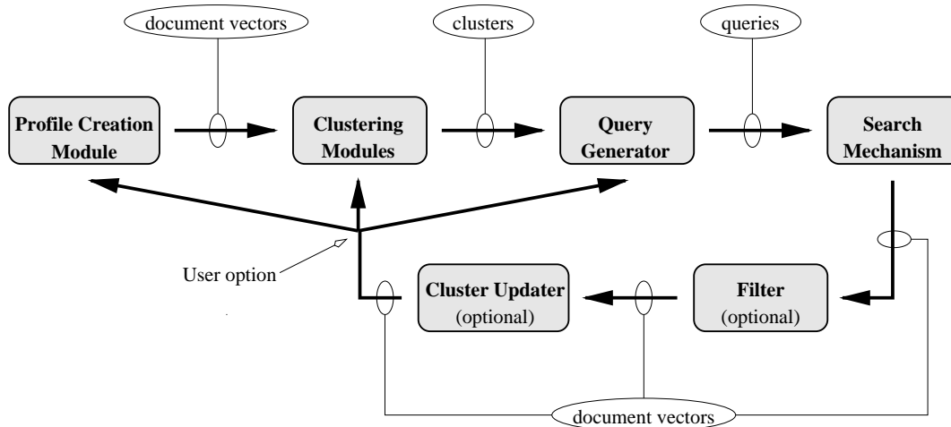
Figure 1: WebACE Architecture
