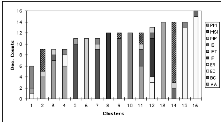
Figure 3: Class distribution of PCA clusters.
